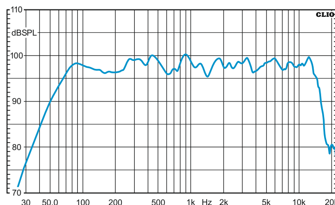
L151 Frequency Response
